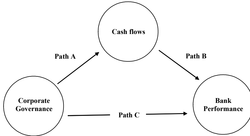
FIGURE 1.— Theoretical Model
